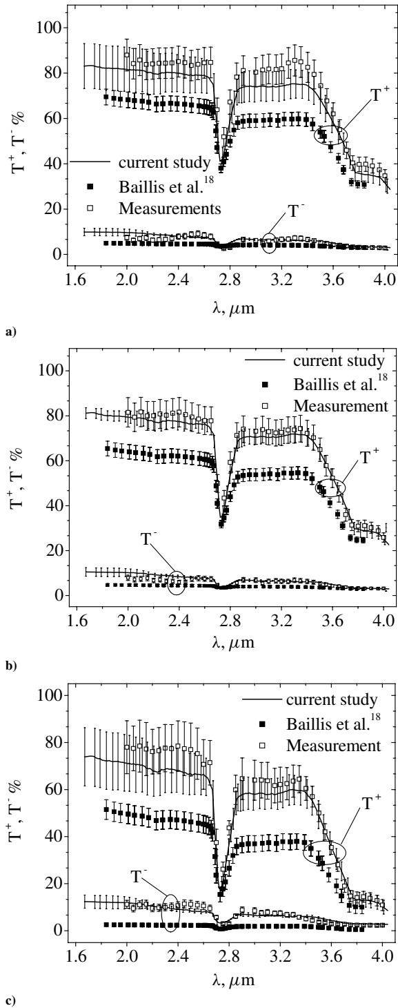
Fig. 10 Comparison between the computed and measured hemispherical transmittance and reflectance for the samples a) e = 5 mm, b) e = 6 mm, and c) e = 9.9 mm.
