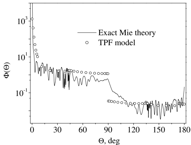
Fig. 2 Mie scattering function of an optically large bubble of size parameter x = 2000 and TPF function characterized by f_1 = 0.2 , g_1 = 0.98 , and g_2 = 0.45 .
