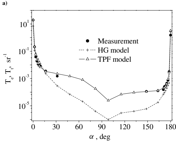
Fig. 8 Influences of the phase function model on the transmittances for the sample e = 6 mm a) at \lambda = 1.89 \mu\text{m} and b) at \lambda = 3.96 \mu\text{m} .
