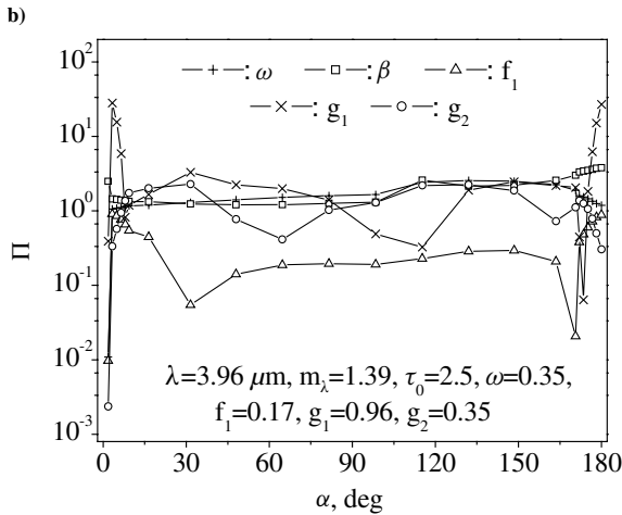
Fig. 6 Dimensionless sensitivity coefficients for a) \lambda = 1.89 \mu\text{m} , b) \lambda = 3.20 \mu\text{m} , and c) \lambda = 3.96 \mu\text{m} .
