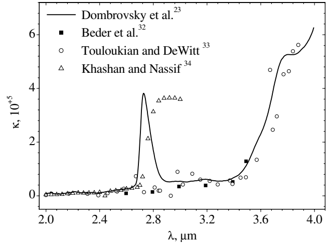
Fig. 4 Index of absorption of fused quartz from literature.
