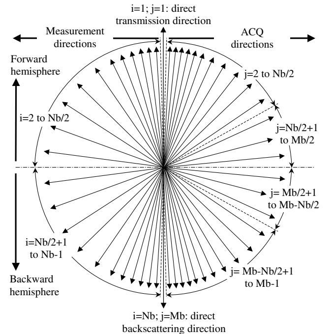
Fig. 3 Measurement and ACQ directions.
