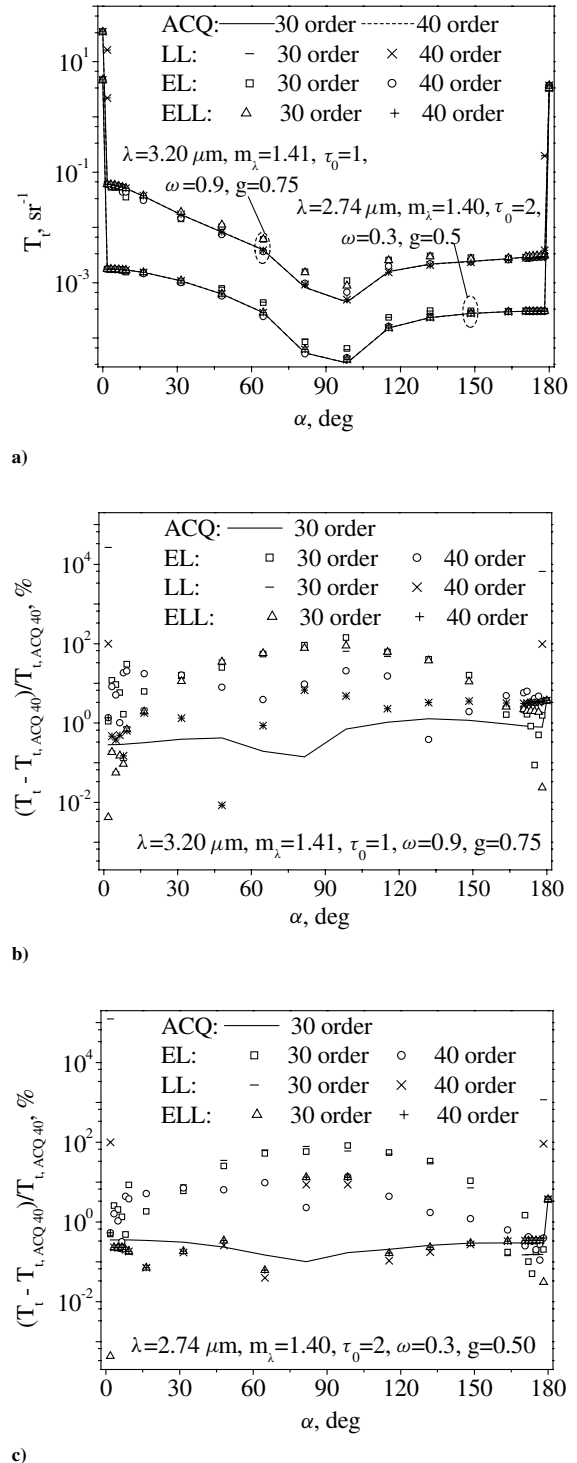
Fig. 5 a) Comparison between transmittances from the interpolation laws (LL, EL, and ELL) and the ACQ; b) relative transmittance deviation of the different interpolation laws (LL, EL, and ELL) compared with the ACQ for \lambda = 3.20 \mu\text{m} ; c) relative transmittance deviation of the different interpolation laws (LL, EL, and ELL) compared with the ACQ for \lambda = 2.74 \mu\text{m} .
