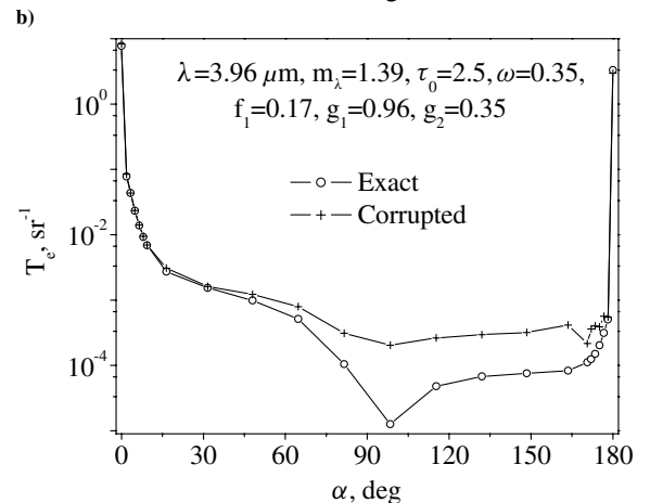
Fig. 7 Simulated exact and corrupted bidirectional transmittances for a) \lambda = 1.89 \mu\text{m} , b) \lambda = 3.20 \mu\text{m} , and c) \lambda = 3.96 \mu\text{m} .
